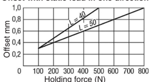
Offset with static load in one direction
