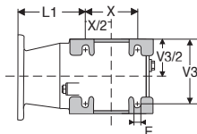
Brackets facing inwards
