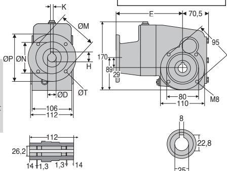
Output shaft
