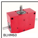
Right angled gearbox, double output shafts, up to 70 Nm
