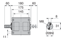
Single output shaft S or dual shafts B
