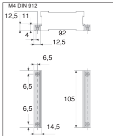
DOMI80-B fastening set
