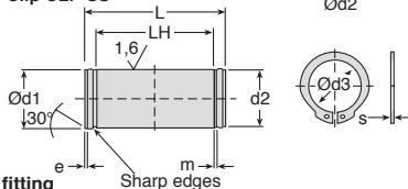
End fitting
