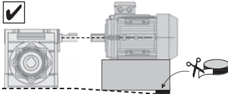
Wedge adjustment
