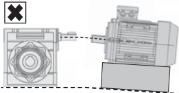
Incorrectly aligned
