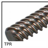
High helix leadscrew, Leadscrew only - up to 40mm per rotation
