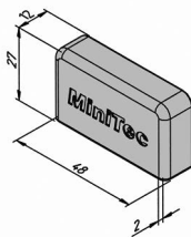
Capuchon PRF45-GOU-C
