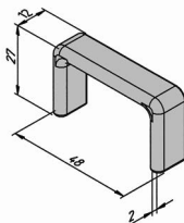
Embout PRF45-GOU-E
