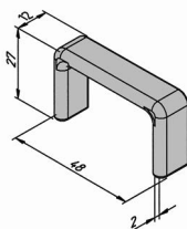
Embout PRF45-GOU-E
